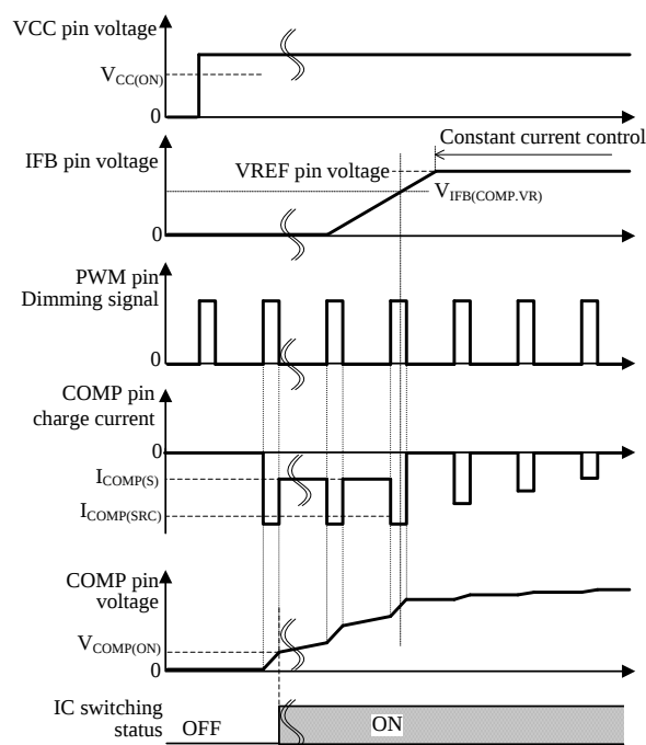
Figure 8-3 Startup operation during PWM dimming
