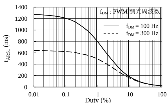
Figure 8-16 PWM dimming on-duty vs. t_{ARS2} (BL020×C)
