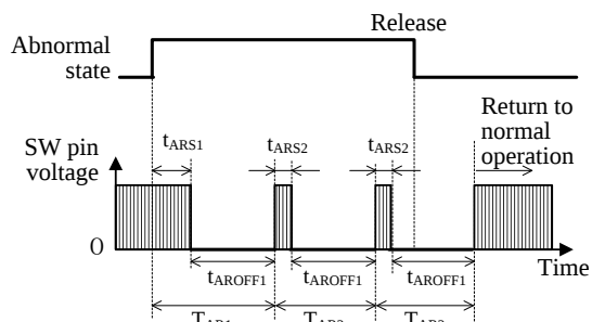
Figure 8-13 Auto Restart 1
