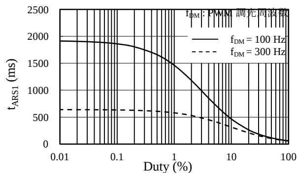
Figure 8-17 PWM dimming on-duty vs. t_{ARS1} (BL0202B)
