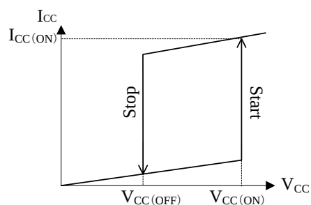
Figure 8-2 V_{CC} versus I_{CC}
