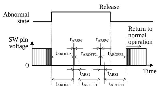
Figure 8-14 Auto Restart 2
