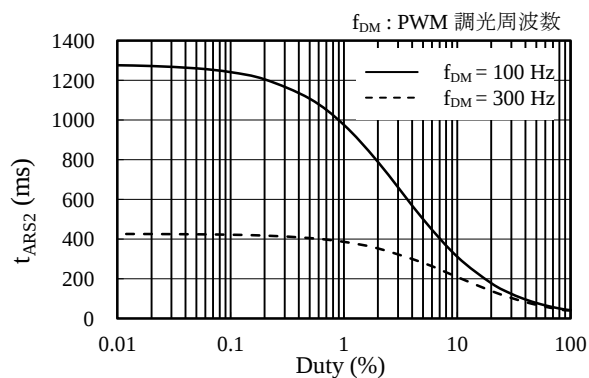
Figure 8-18 PWM dimming on-duty vs. t_{ARS2} (BL0202B)
