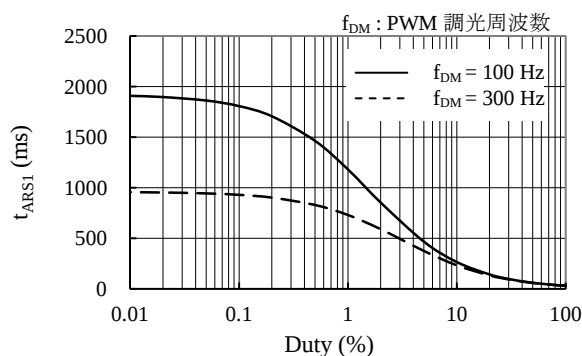
Figure 8-15 PWM dimming on-duty vs. t_{ARS1} (BL020×C)
