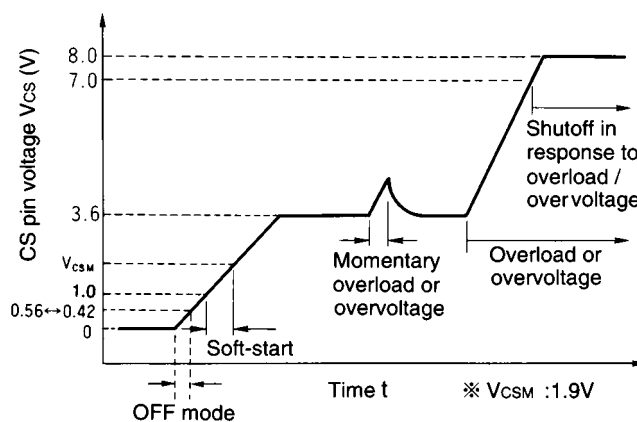
Fig. 6 CS pin waveform
