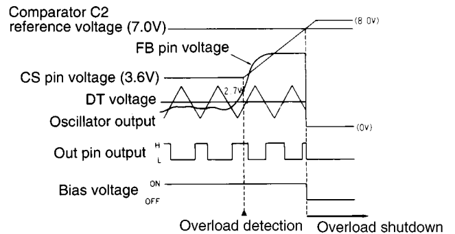
Fig. 10 Overload shutdown timing chart
