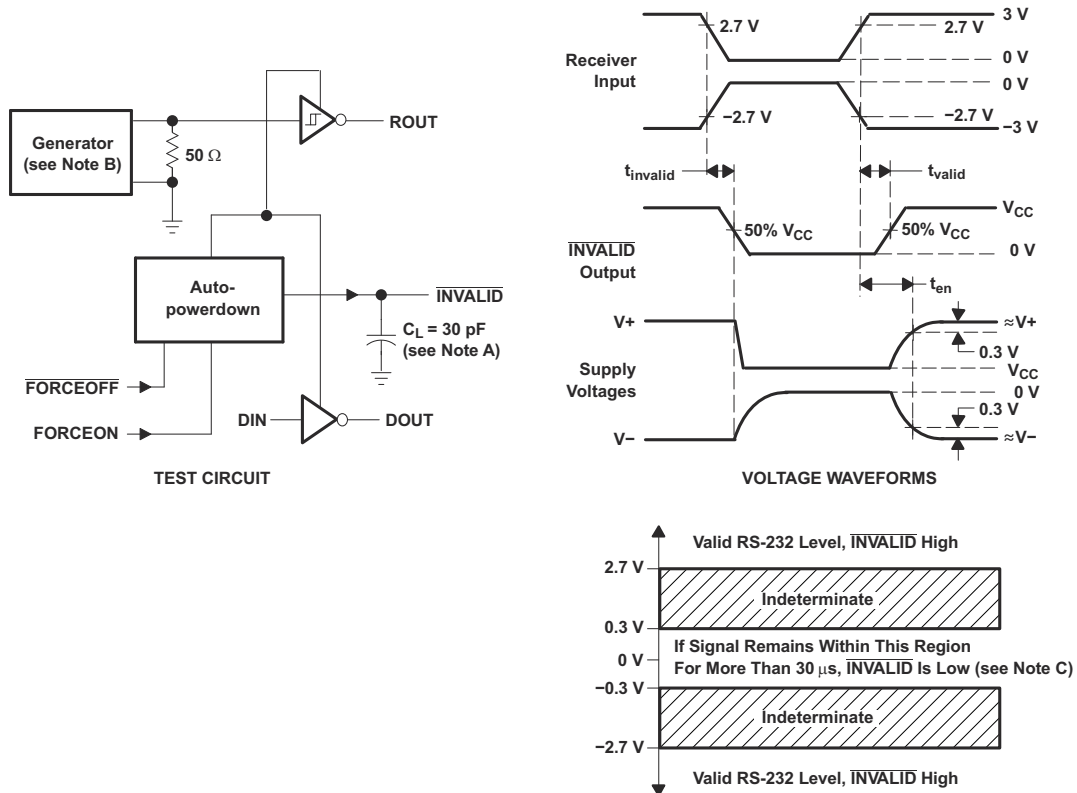
Figure 7-4. Receiver Enable and Disable Times
