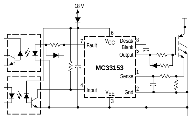
Figure 37. Sense IGBT Application
