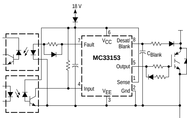
Figure 36. Desaturation Application
