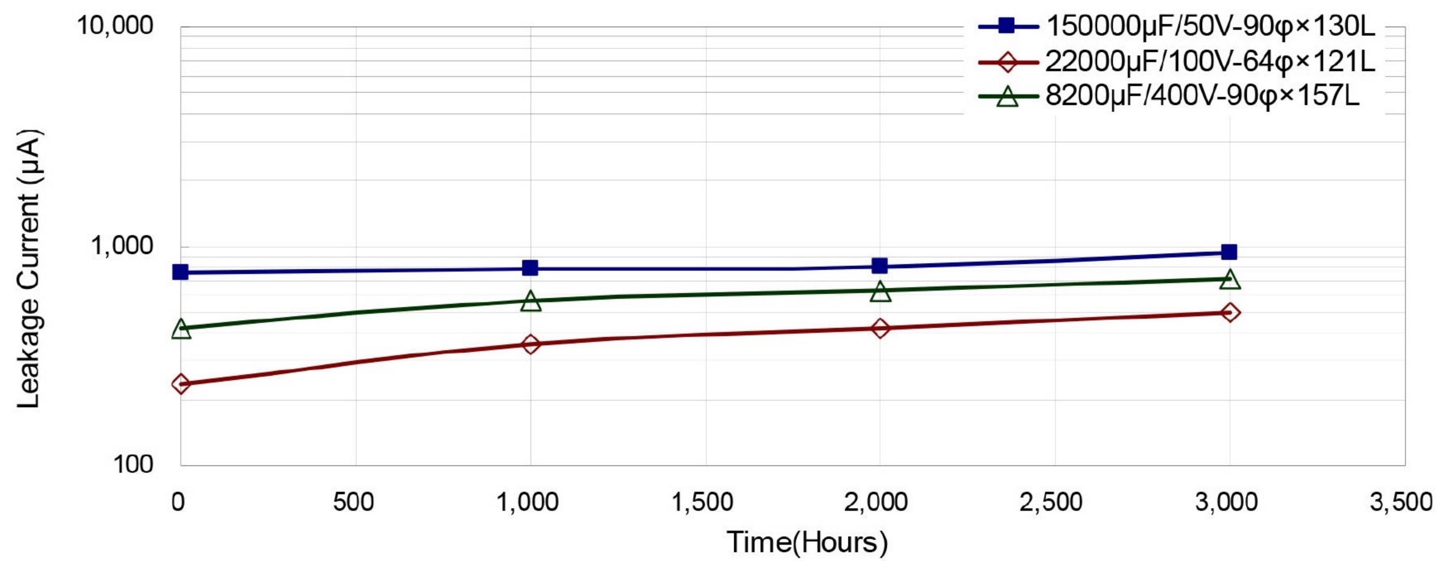
Useful Life Chart
