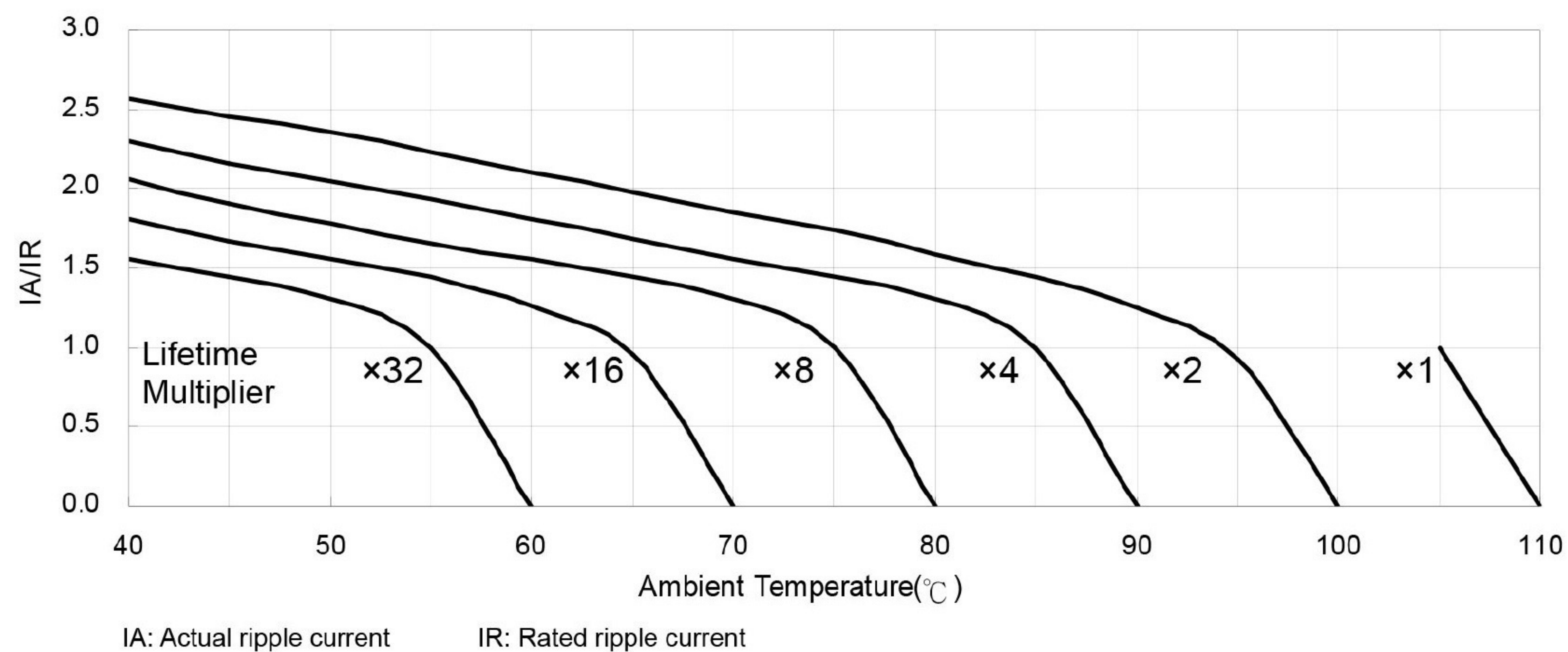
Useful Life Chart
