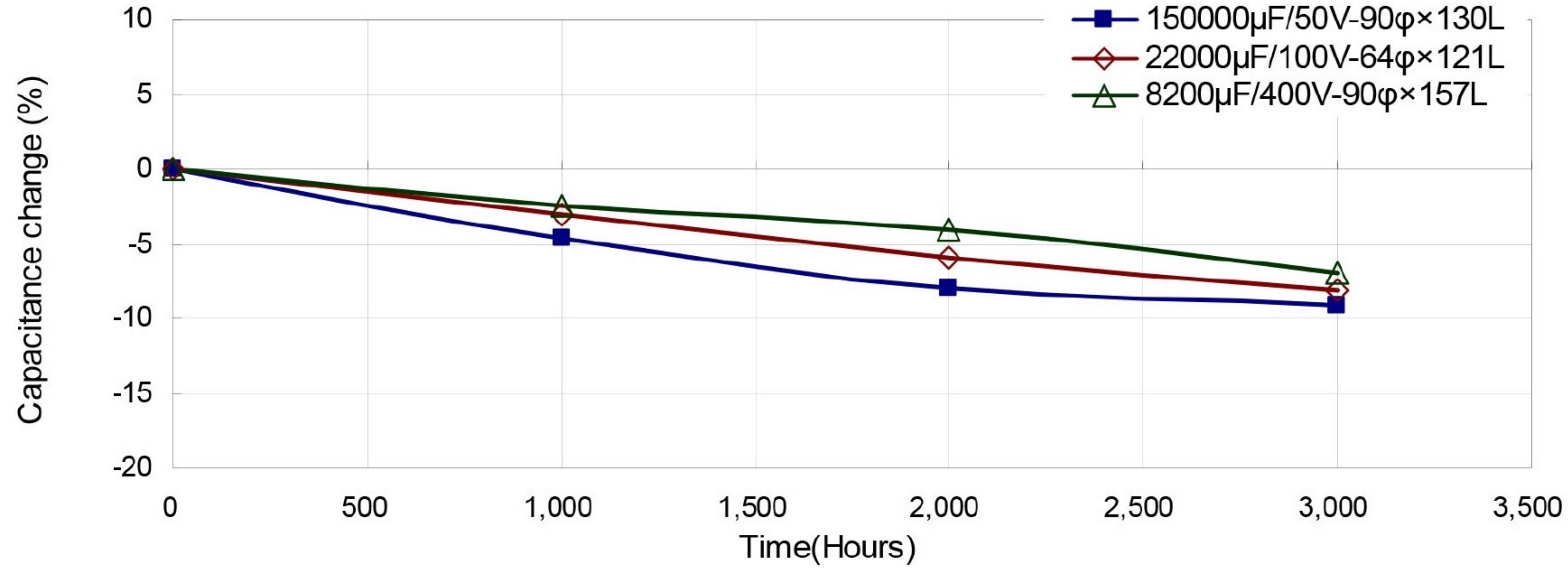
Typical Endurance Curves
