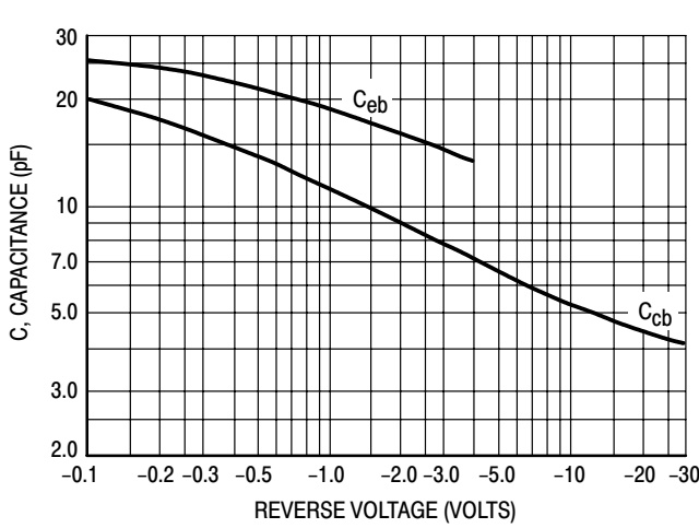
Figure 9. Capacitances
