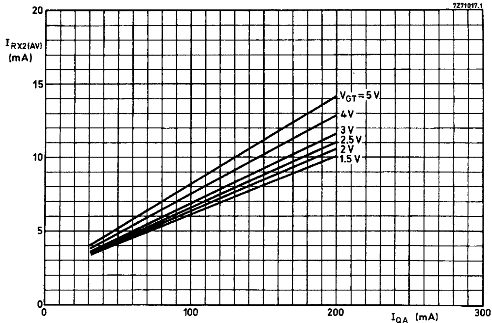
Fig.4 Average supply current I_{RX2(AV)} as a function of output current I_{QA} with triac gate trigger voltage V_{GT} as a parameter; typical performance.
