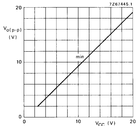
Fig. 9 Minimum values of the output voltage swing as a function of supply voltage for R_L = 1 kΩ.
