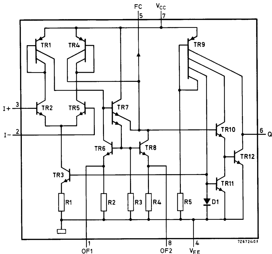
Fig. 1 Circuit diagram.
