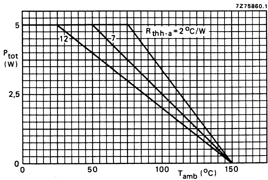
Fig.2 Total power dissipation. The graph takes into account an R_{th\ tab-h} = 1\ ^{\circ}\text{C/W} which is to be expected when the tab is connected to a heatsink with one 3 mm bolt, without using heatsink compound. R_{th\ j-tab} = 12\ ^{\circ}\text{C/W} .
