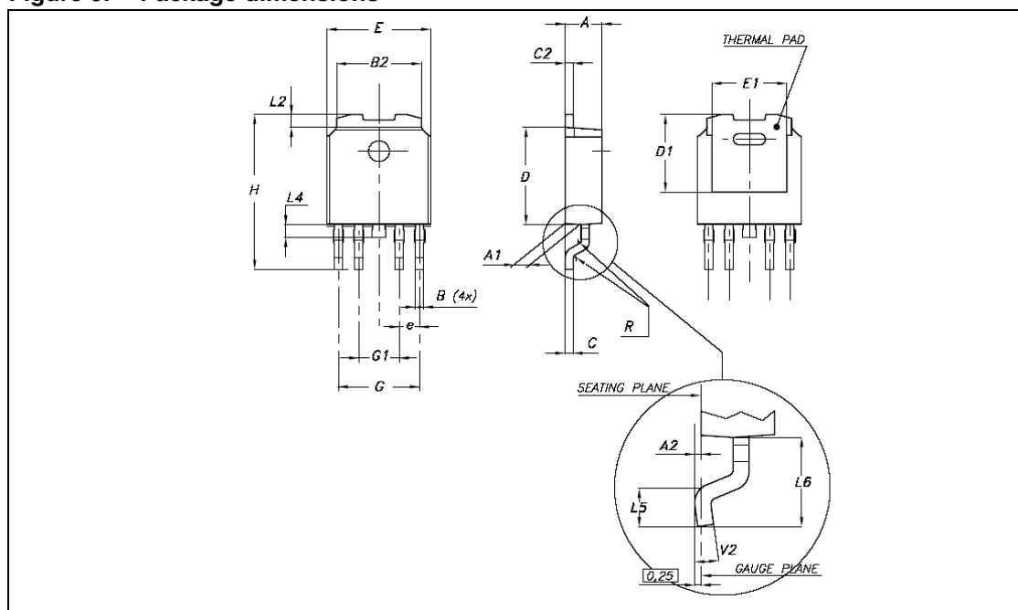
Figure 9. Package dimensions
