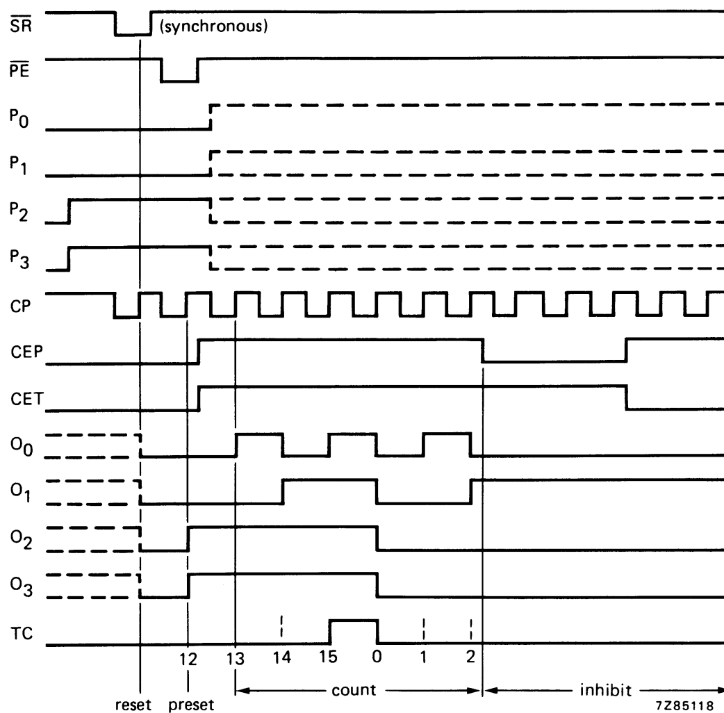
Fig.9 Timing diagram.
