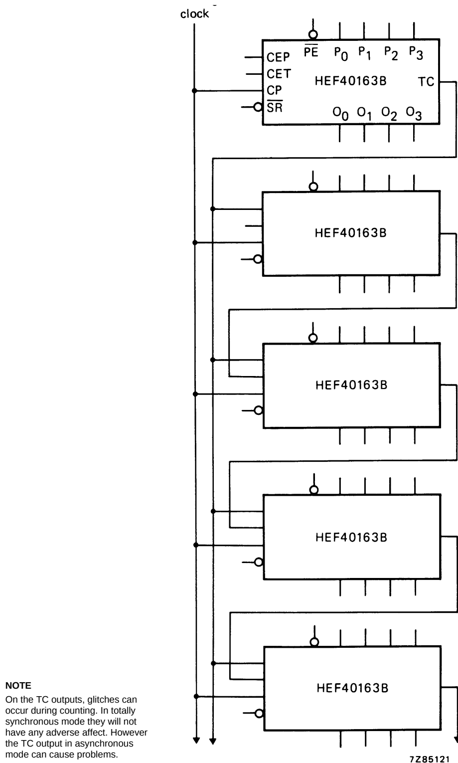
Fig.10 Synchronous multi-stage counting scheme.
